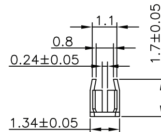
C-C SEC
