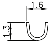
B-B SEC
