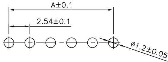
Recommened PCB Layout
