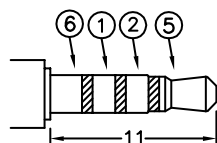
Recommended 2.5 mm \phi Mating Plug
