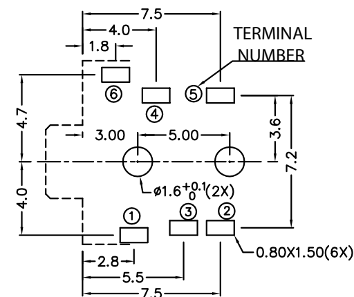
RECOMMENDED PCB LAYOUT (BOTTOM VIEW)
