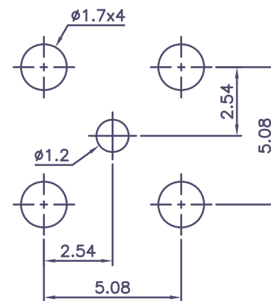
RECOMMENDED PCB LAYOUT DIMENSIONS
