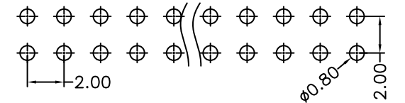
Recommended P.C.B Layout(Top Side)
