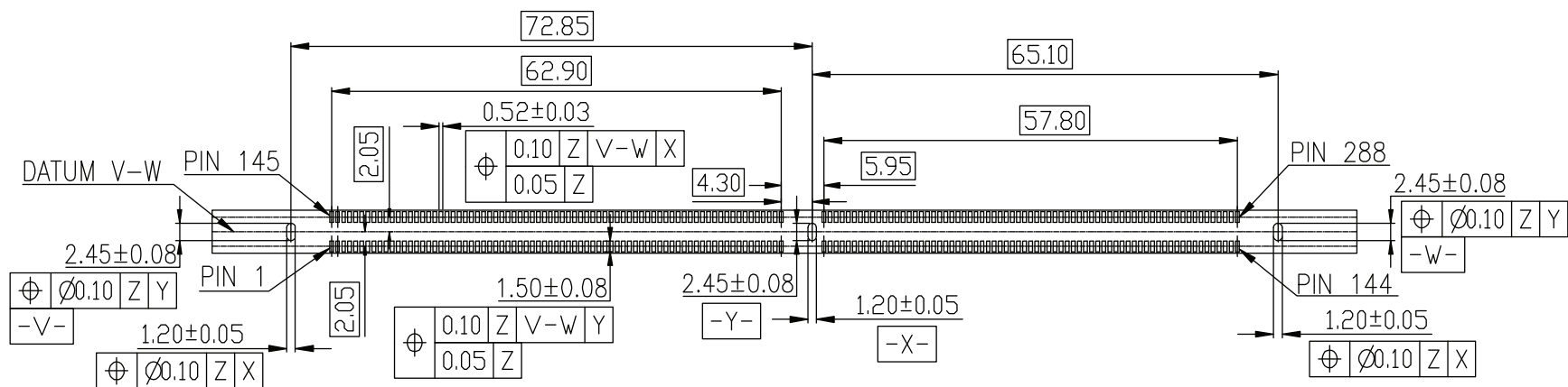
RECOMMENDED PC BOARD LAYOUT (TOP VIEW)
