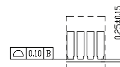
DETAIL C SCALE 1:4
