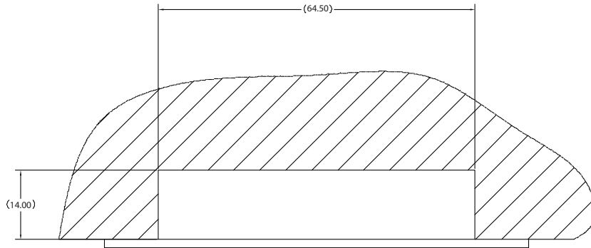
PANEL CUT-OUT
