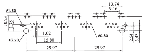
PCB LAYOUT
